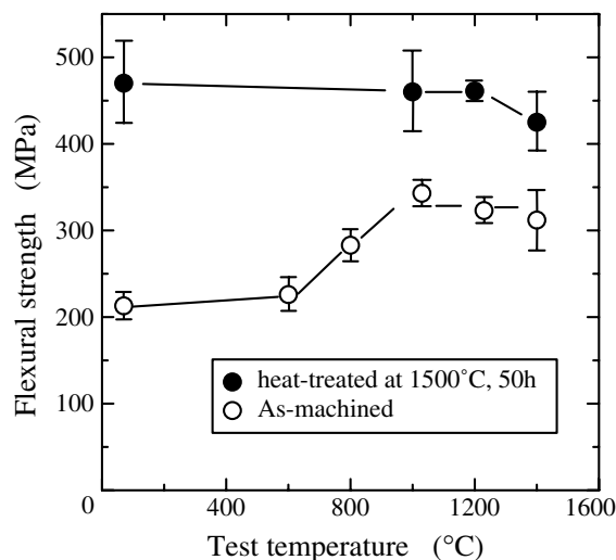
Fig. 3 High temperature strength of silicon carbide ground with 127-μm diamond grit wheel before and after heat treatment in air
