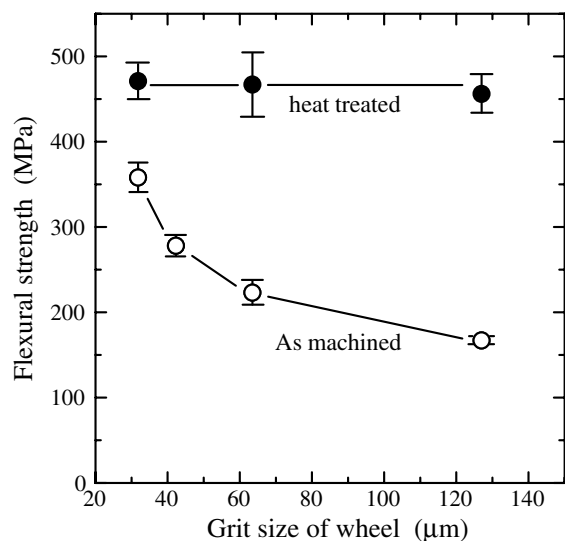
Fig. 2 Influence of heat treatment on flexural strength of silicon carbide ground with various grit sizes of wheel
