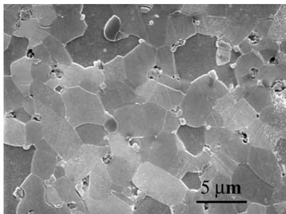
Fig. 1 Microstructure of silicon carbide
